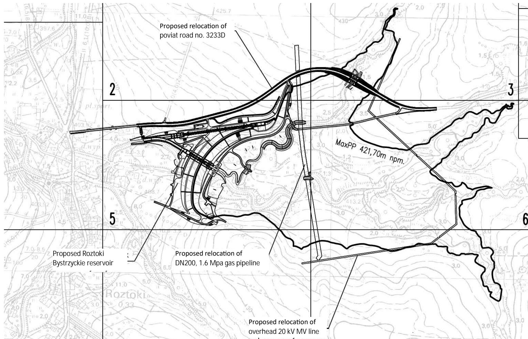
Map 1 Location of "Roztoki Bystrzyckie" - a dry flood control reservoir on Goworówka stream
