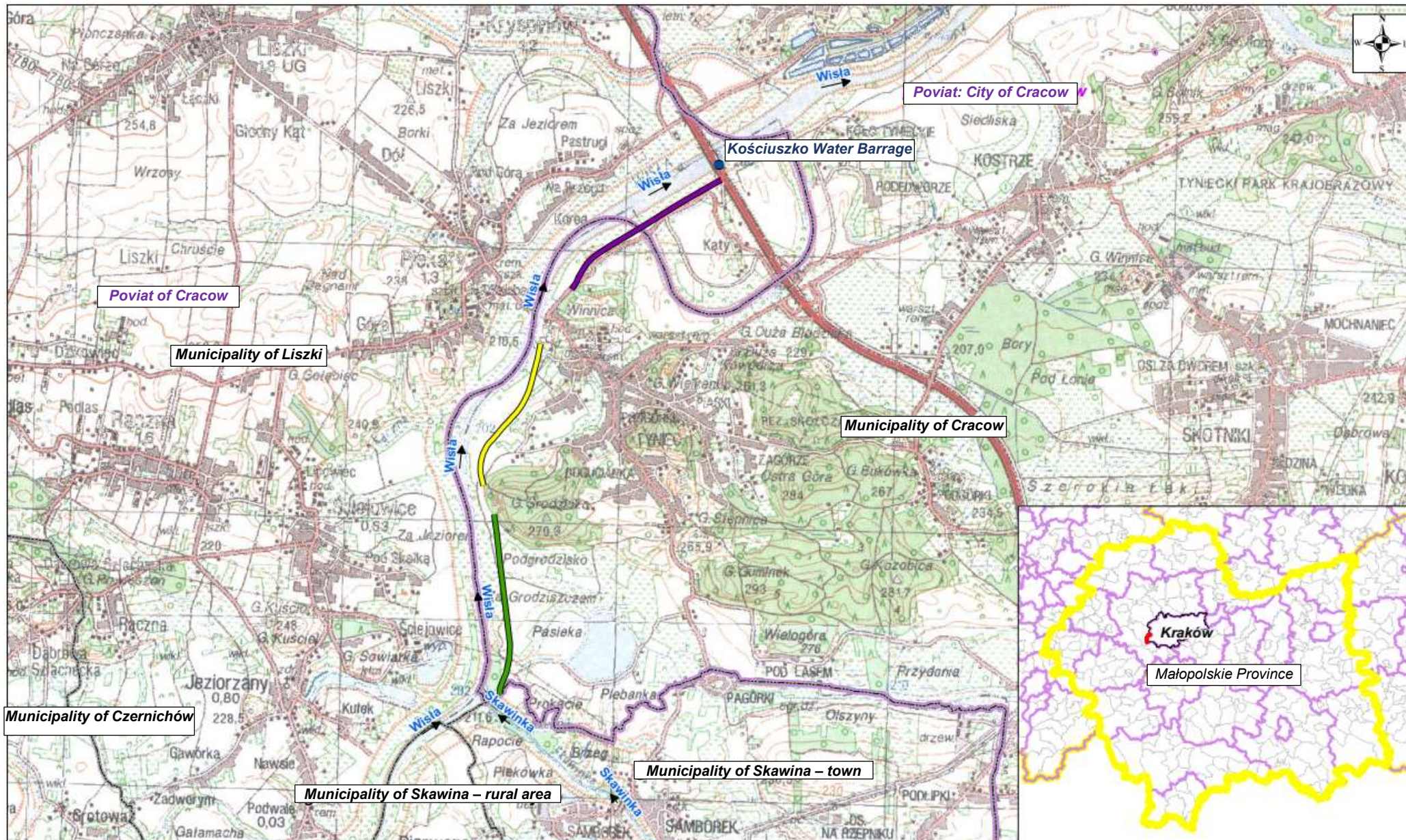
Appendix 1 – Location of Works Contract 3A.3 Section 4 – The right embankment of the Vistula River from the estuary of Skawinka to the Kościuszeko barrage.
