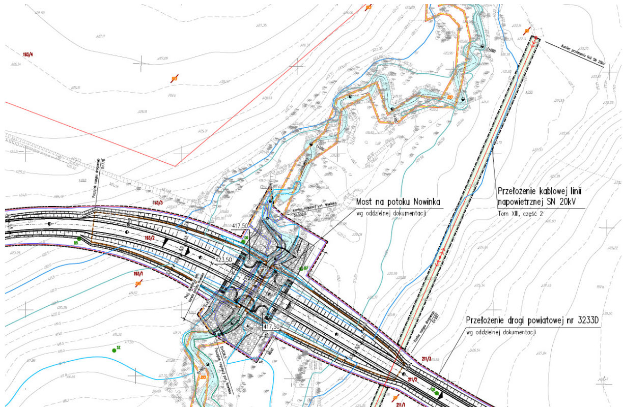
Map 2 – Location of designed bridge on the Nowinka stream with designed relocation of a 20 kV MV overhead power cable line, and designed relocation of district road 3233D. Northeastern area of the project.
