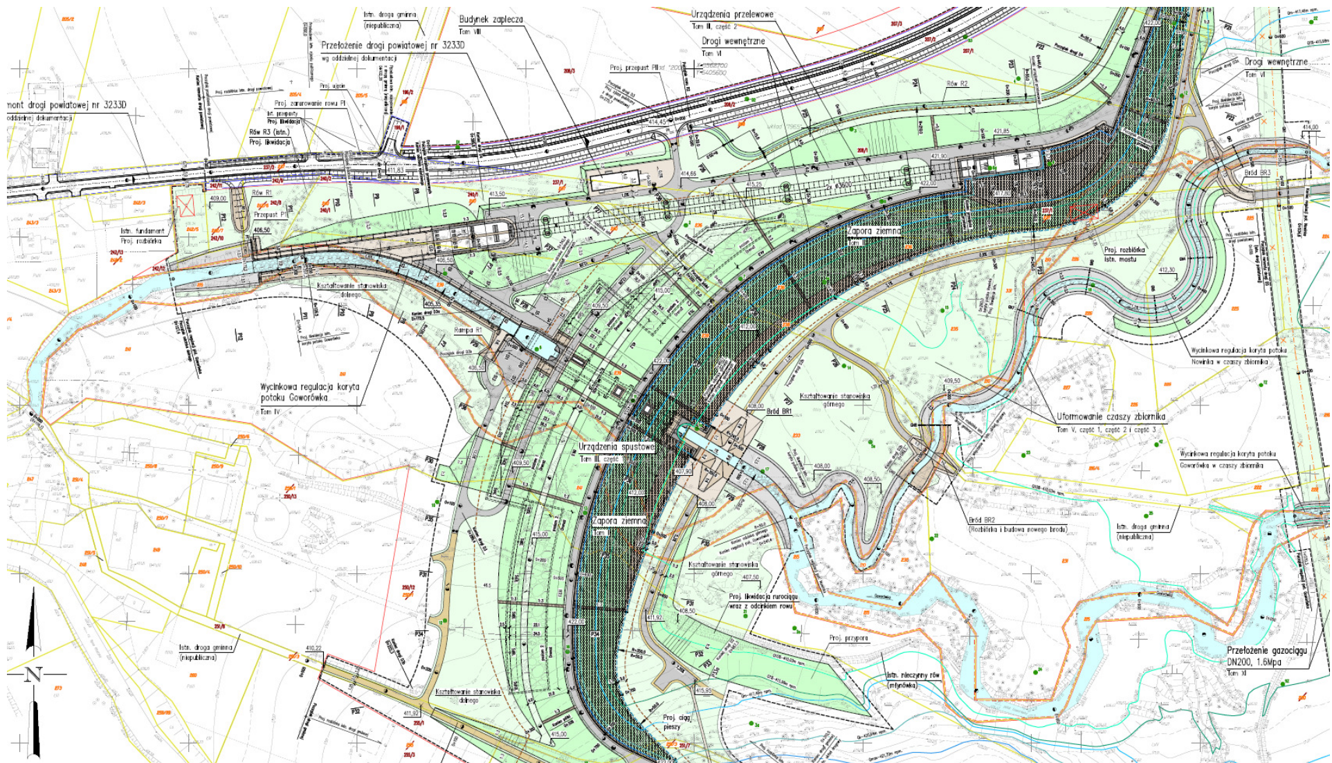
Map 3 – Location of the earth-fill dam
